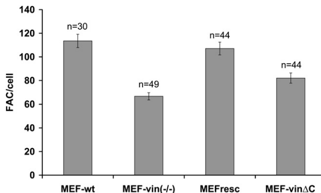
FIGURE 4 Numbers of focal adhesions (FAs) per cell determined from confocal microscopic images. Only cells of similar spreading area ( \sim 4000 \mu\text{m}^2 ) were analyzed, showing ~115 FAs in MEF-wt, 65 FAs in MEF-vin(-/-), 110 FAs in MEF-resc, and 82 FAs in MEF-vinΔC cells. Note that n is the number of cells measured, and that the error bars denote the mean \pm SE.
